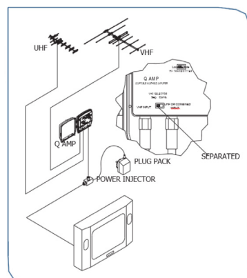
Installation Layout
